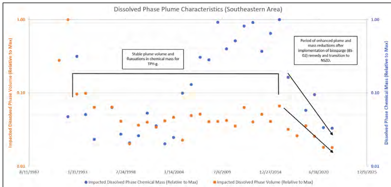
Exhibit 7. Dissolved-phase Plume Characteristics for TPH-g (Southeastern Area) Over Time, Set at an Iso-concentration Value of >100 µg/L, Representative of Saturated Soils in the Subsurface.
